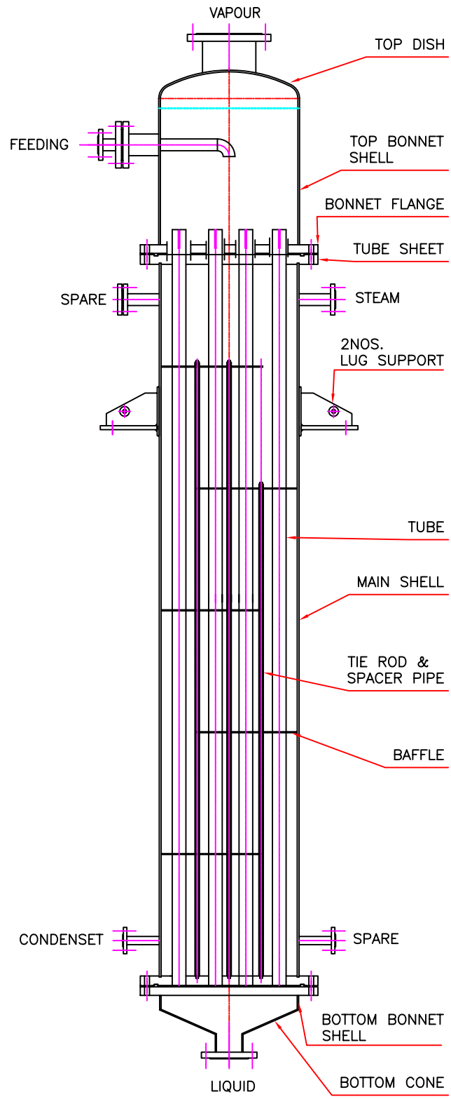
FALLING FILM EVAPORATOR
